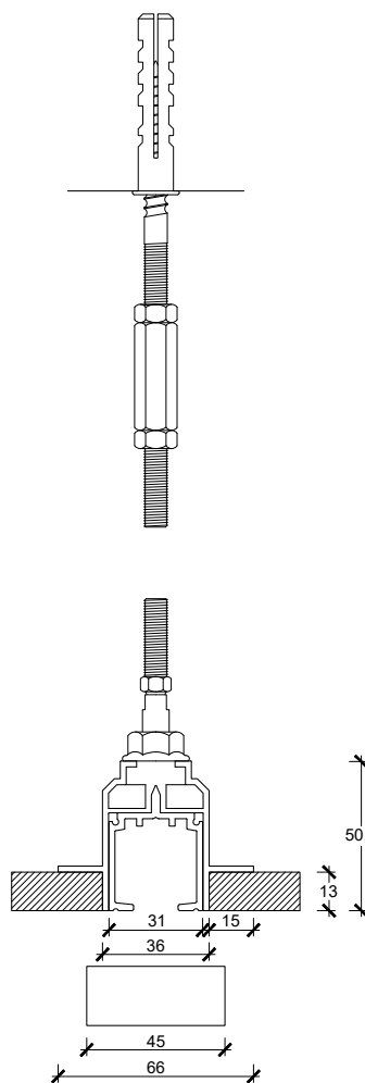
Mounting system for ceiling/ System mocowania do sufitu
