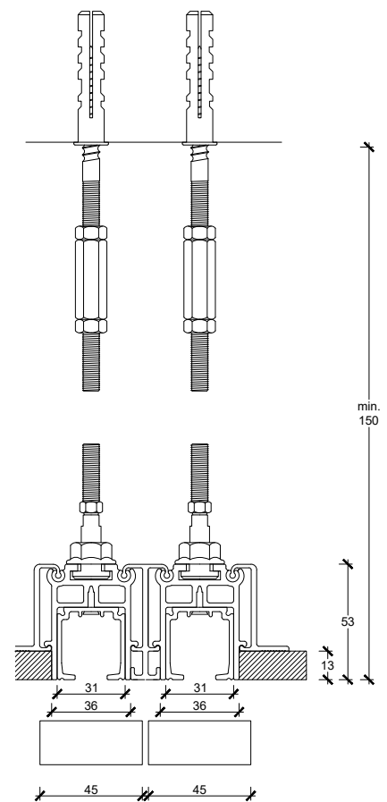
Mounting system for ceiling/ System mocowania do sufitu
